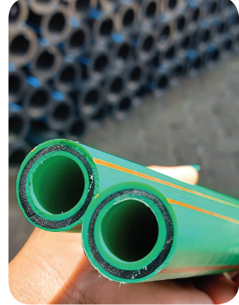
■ Glass-reinforced pipes
